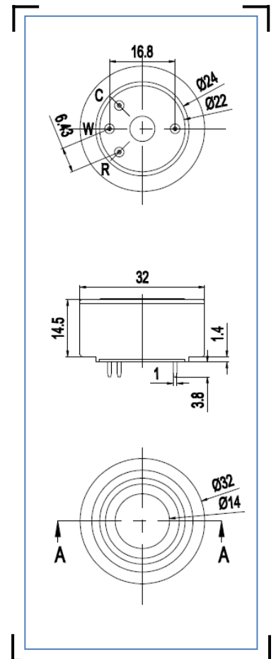
Fig1.Sensor Structure
