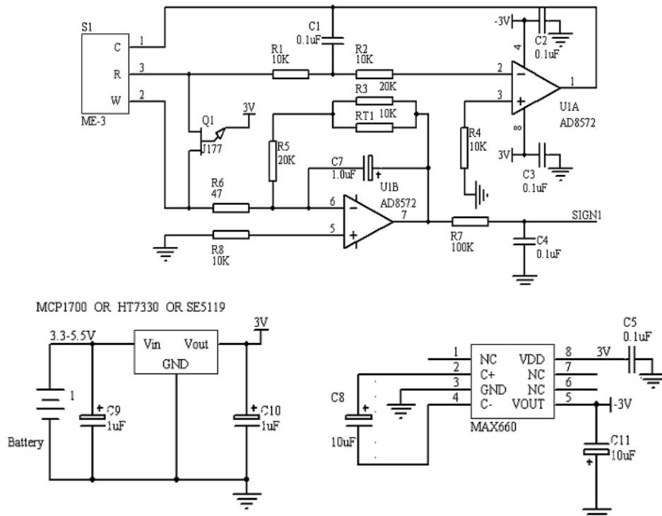
Fig2: MQ-E4 2 H 2 test circuit
