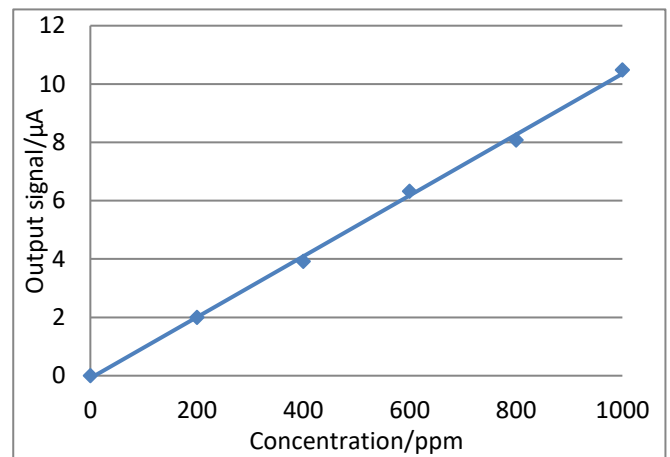
Fig4. Linearity
