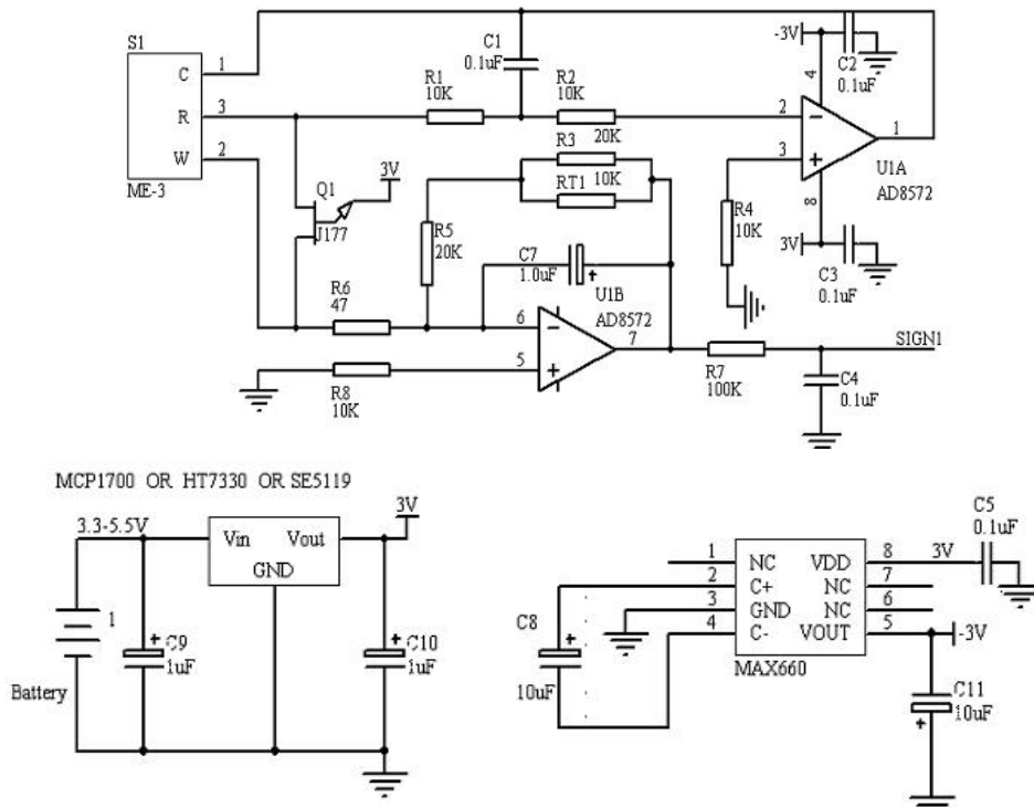
Fig2: MQ-E4-NO 2 test circuit
