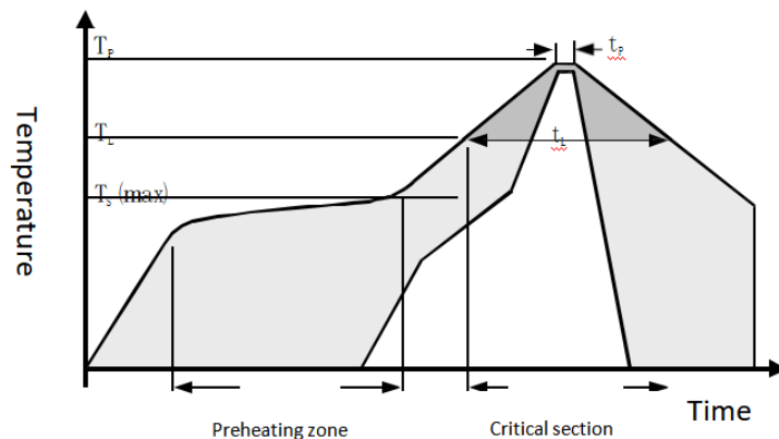
Figure 9: JEDEC standard welding process diagram, T_p \leq 260\text{ °C} , t_p < 30\text{ sec} , lead-free soldering. T_L < 220\text{ °C} , t_L < 150\text{ sec} , the temperature rise and fall speed during welding should be < 5\text{ °C/sec} .
