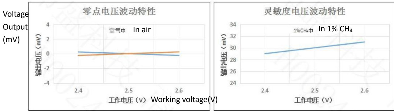
Fig10.Sensitivity with different voltage
