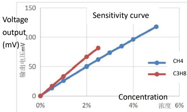
Fig3. Sensitivity Curve
